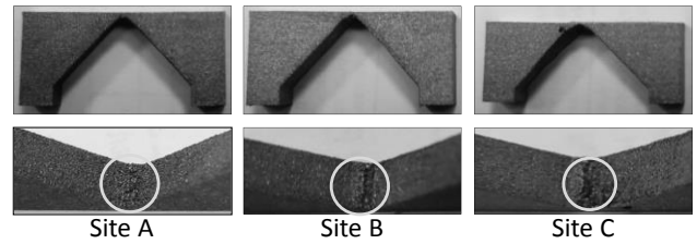
Fig. 9. Residual stress arches highlighting burning marks on the downward surface
