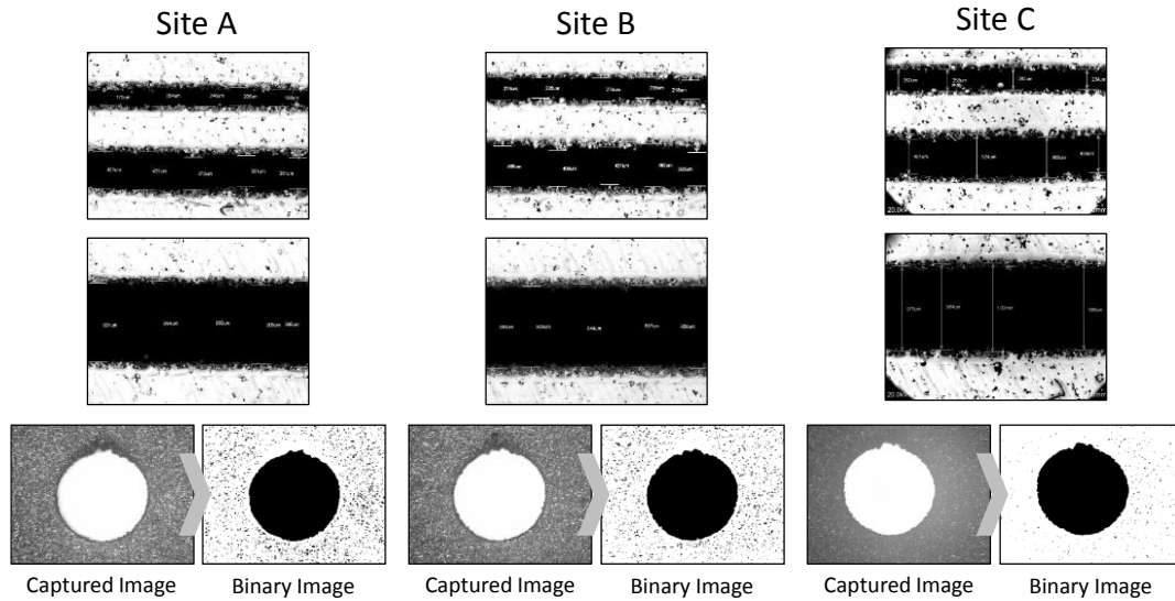
Fig. 7. SEM measurements and image analysis for circle accuracy measurement
