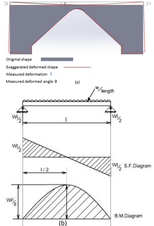
Fig. 4. (a) Exaggerated effect of residual stress on the deformation on the arch, and (b) Simply supported beam with a constant load applied and its corresponding shear force and bending moment diagrams
