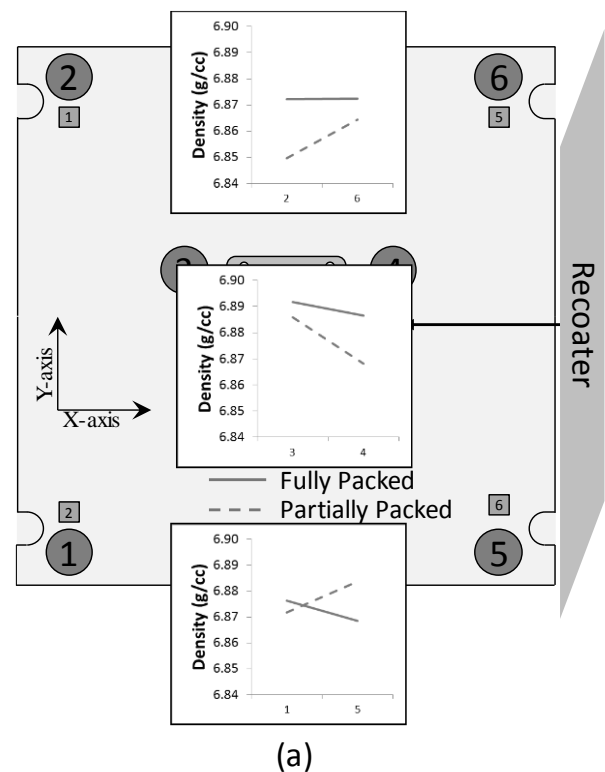
Fig. 11. Partial packed dispenser
