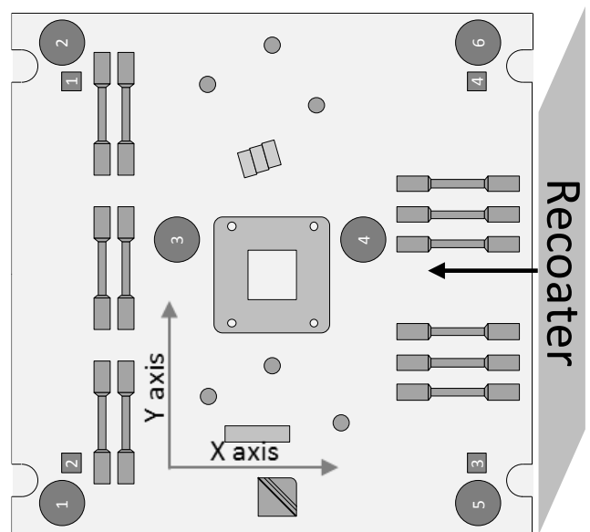
Fig. 2. Build Plate Layout
