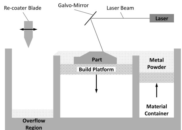
Fig. 1 Schematic diagram of L-PBF Process (image courtesy of Quinn et al. (2019a))
