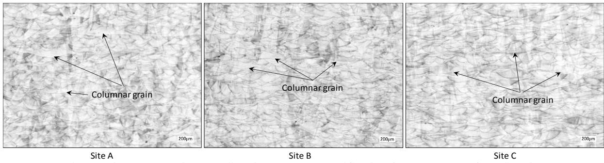
Fig. 6. Microstructure in the z-direction at x200 magnification from each manufacturing site
